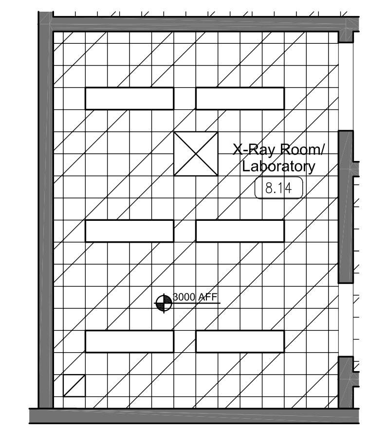
2A REFLECTED CEILING PLAN 1:50
