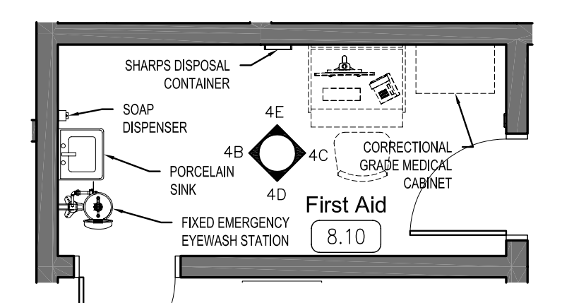
4 HCU FIRST AID ROOM - ENLARGED PLAN 1:50
