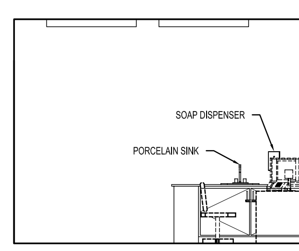
2D ELEVATION 1:50
