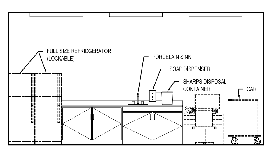
1D ELEVATION 1:50
