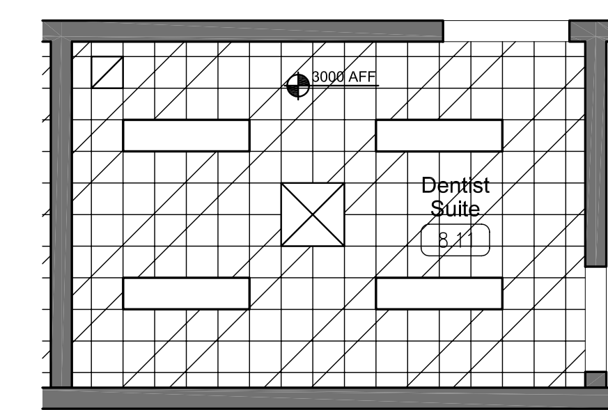
3A REFLECTED CEILING PLAN 1:50
