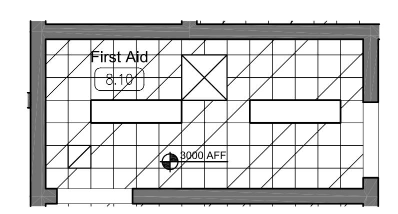
4A REFLECTED CEILING PLAN 1:50
