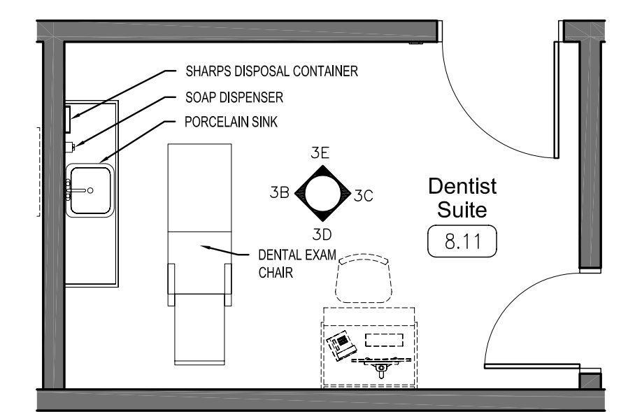
3 DENTIST SUITE - ENLARGED PLAN 1:50
