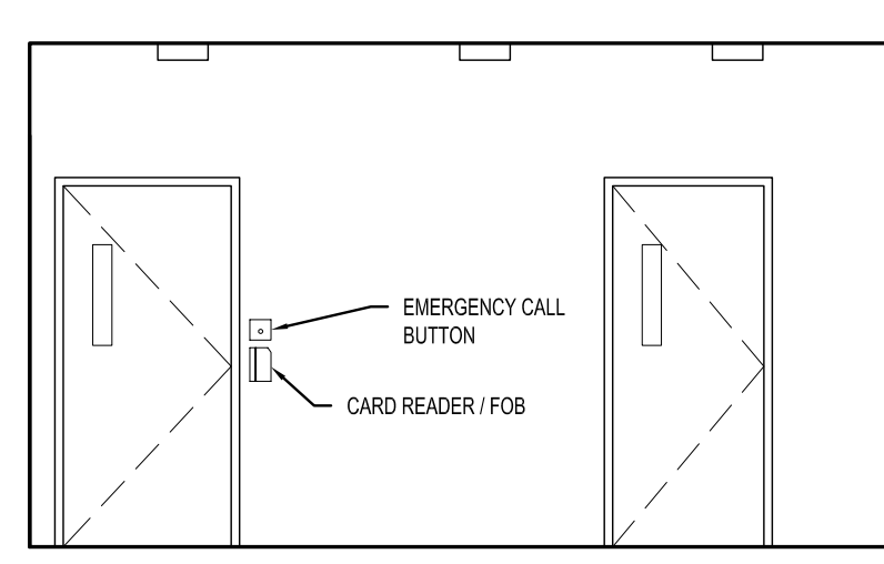
2C ELEVATION 1:50
