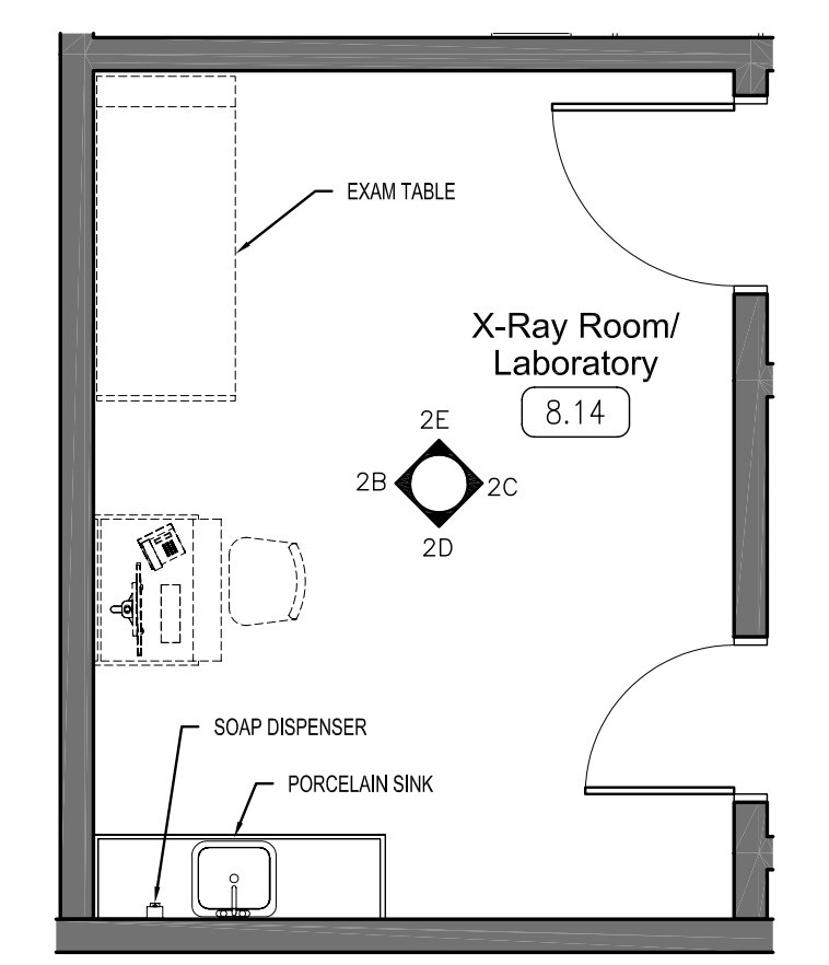
2 X-RAY ROOM - ENLARGED PLAN 1:50
