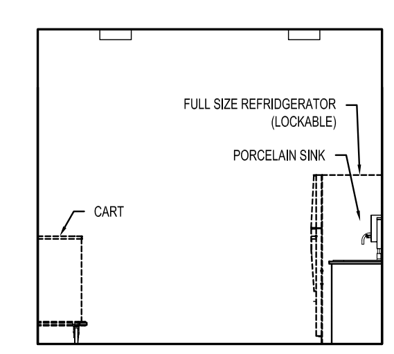
1C ELEVATION 1:50
