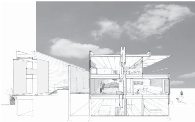
longitudinal section through unit
