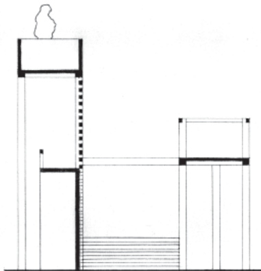
section b-b
