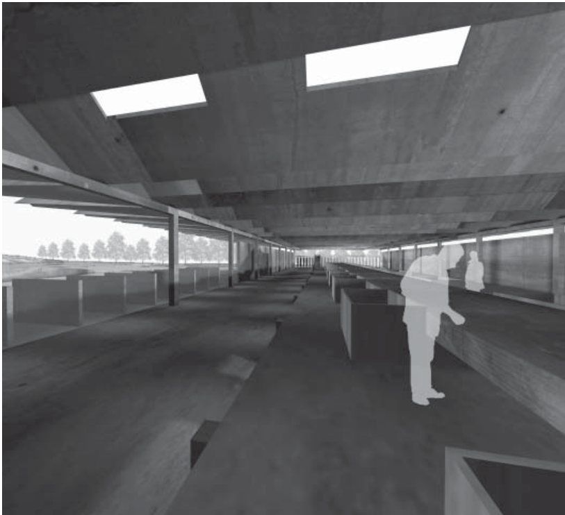
interior of center looking down the longitudinal axis of the sorting line. operable glazed facade to the north allows views to the working yard beyond.
