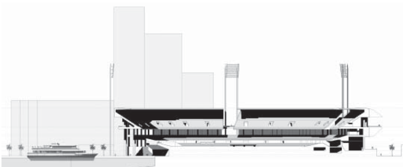
site section
