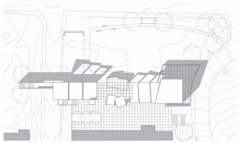
site plan
