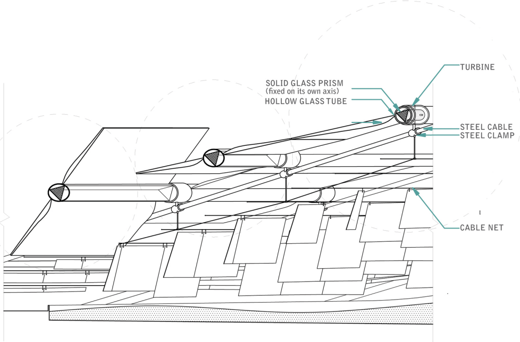
STRUCTURAL DETAIL
