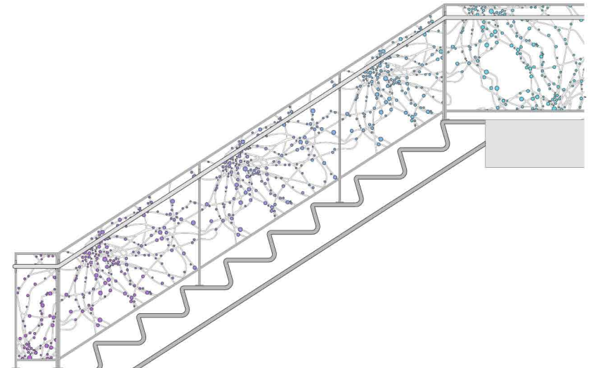
STAIR SECTION
