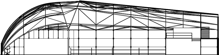
TRANSVERSE SECTION
