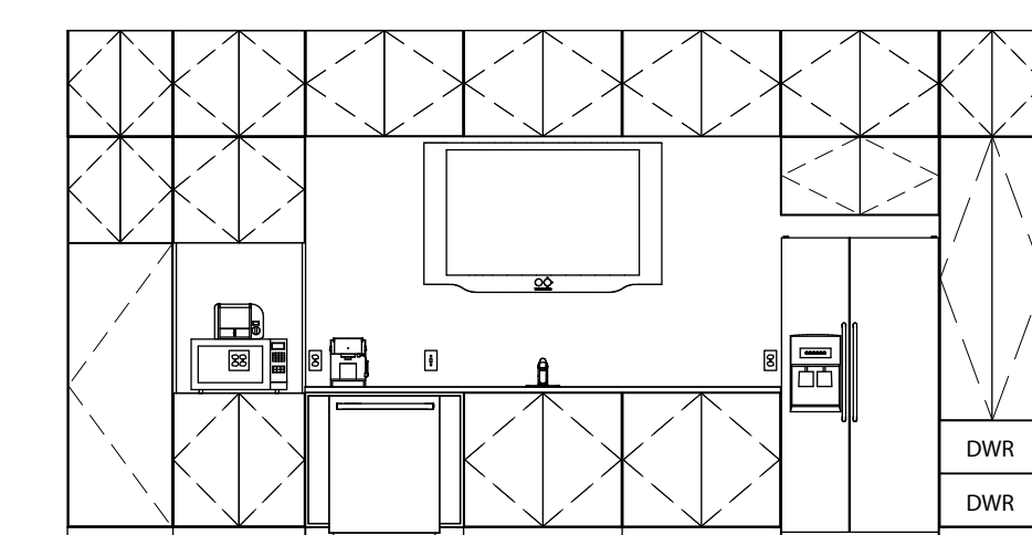
INTERIOR ELEVATION DETAIL 3 1/4"=1'-0"
