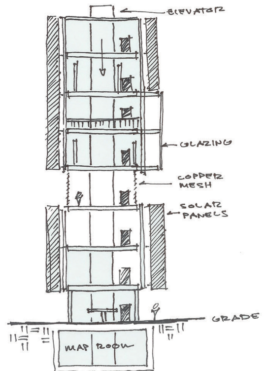
East/West Section
