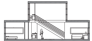
typ. 3/5 bedroom transverse section
