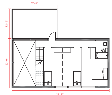
typ. 3/5 bedroom second level plan
