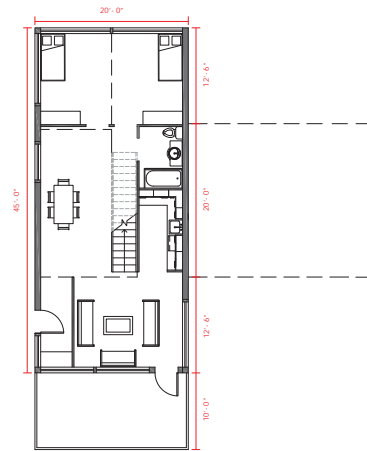
typ. 3/5 bedroom first level plan
