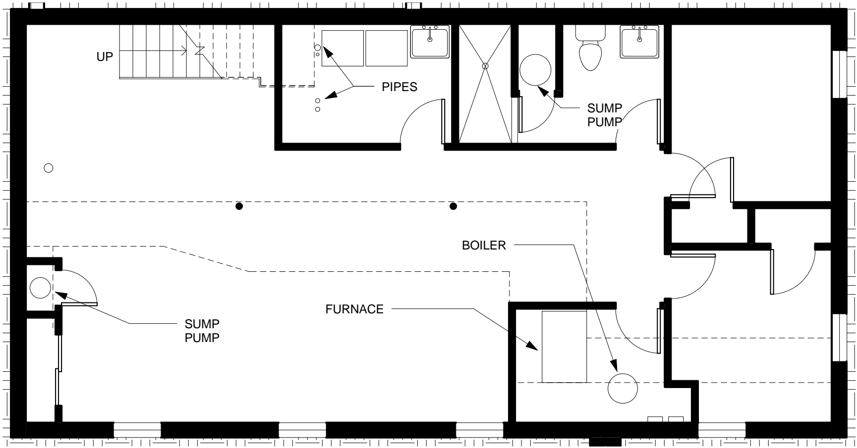
1 Basement - Enlarged 3/16" = 1'-0"
