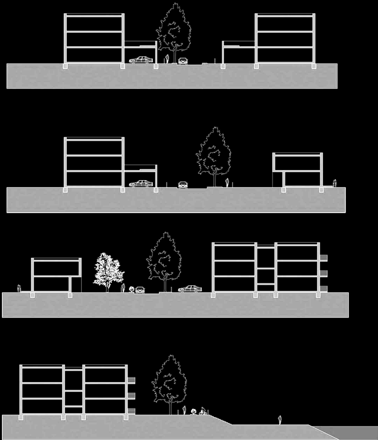
STREET SECTIONS
