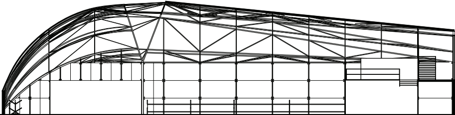
TRANSVERSE SECTION
