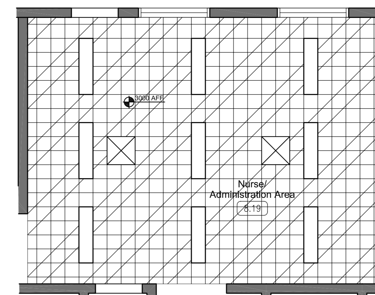
1A REFLECTED CEILING PLAN 1:50
