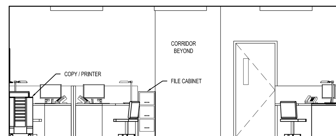
1D ELEVATION 1:50
