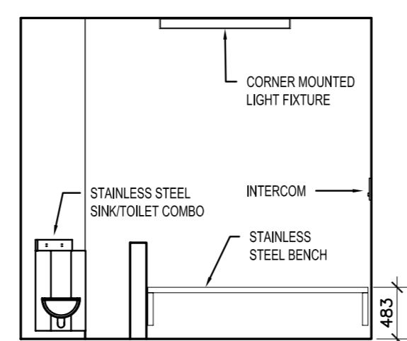
5D ELEVATION 1:50
