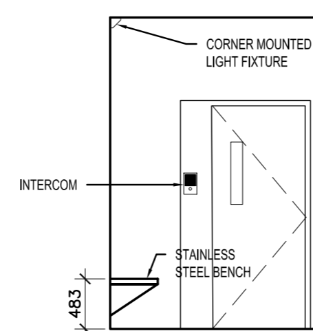
5C ELEVATION 1:50
