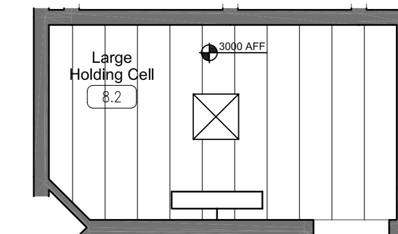
4A REFLECTED CEILING PLAN 1:50
