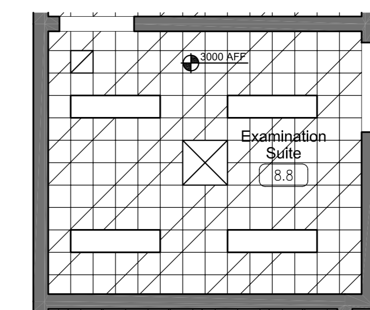
2A REFLECTED CEILING PLAN 1:50
