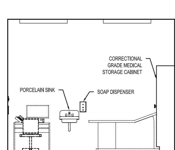
2D ELEVATION 1:50
