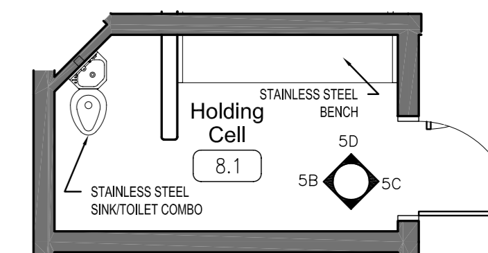
5 HCU HOLDING CELL - ENLARGED PLANS 1:50
