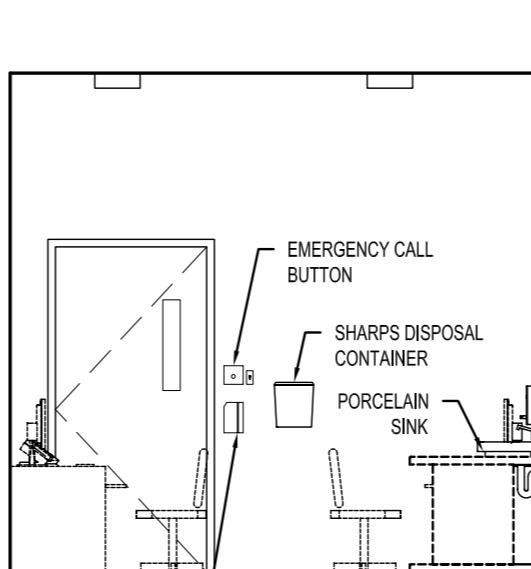
2C ELEVATION 1:50
