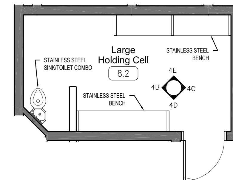
4 HCU LARGE HOLDING CELL - ENLARGED PLANS 1:50
