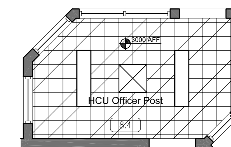
3A REFLECTED CEILING PLAN 1:50
