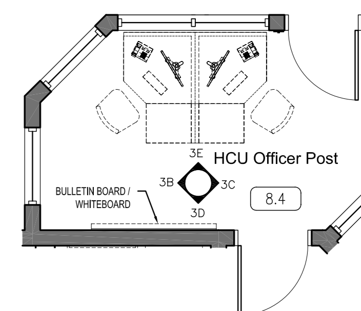
3 HCU OFFICER POST - ENLARGED PLANS 1:50
