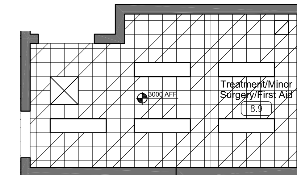
1A REFLECTED CEILING PLAN 1:50
