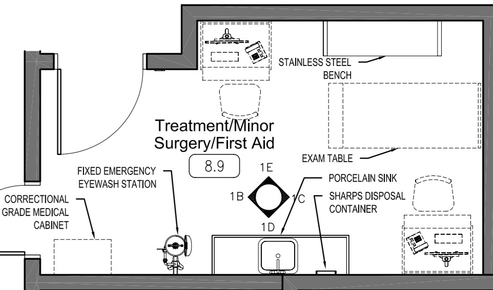
1 TREATMENT/MINOR SURGERY/FIRST AID ENLARGED PLANS 1:50
