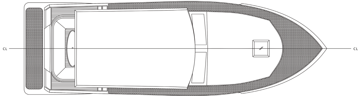
DECK PLAN/LAYOUT
