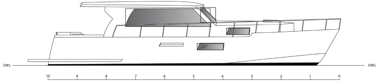
OUTBOARD PROFILE
