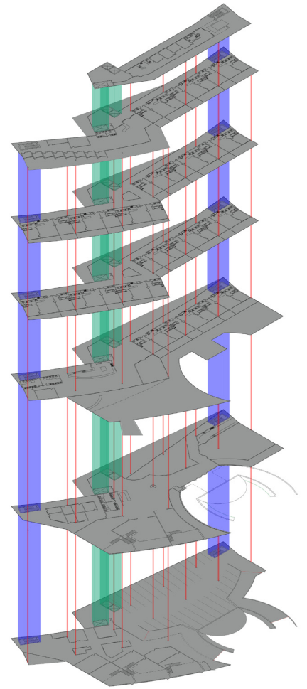
Structural Perspective
