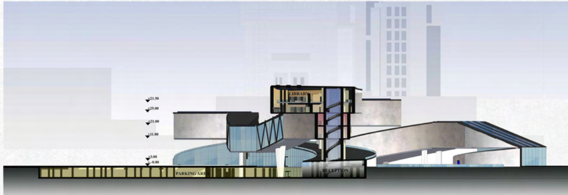
SECTION F-F SCALE 1/200
