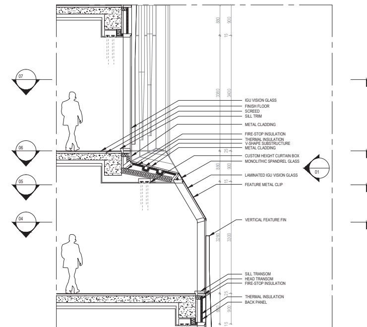
02 TYPICAL EWS02A FACADE TYPE - PARTIAL SECTION
