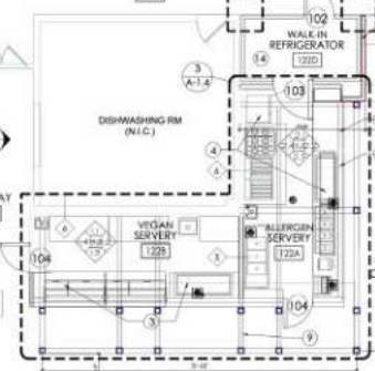
KITCHEN DESIGN WITH EQUIPMENT LAYOUT
