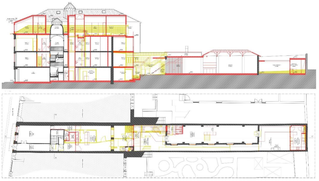
Demolition and Construction drawings CAD (Rehabilitation of a historical typology house in Porto)
