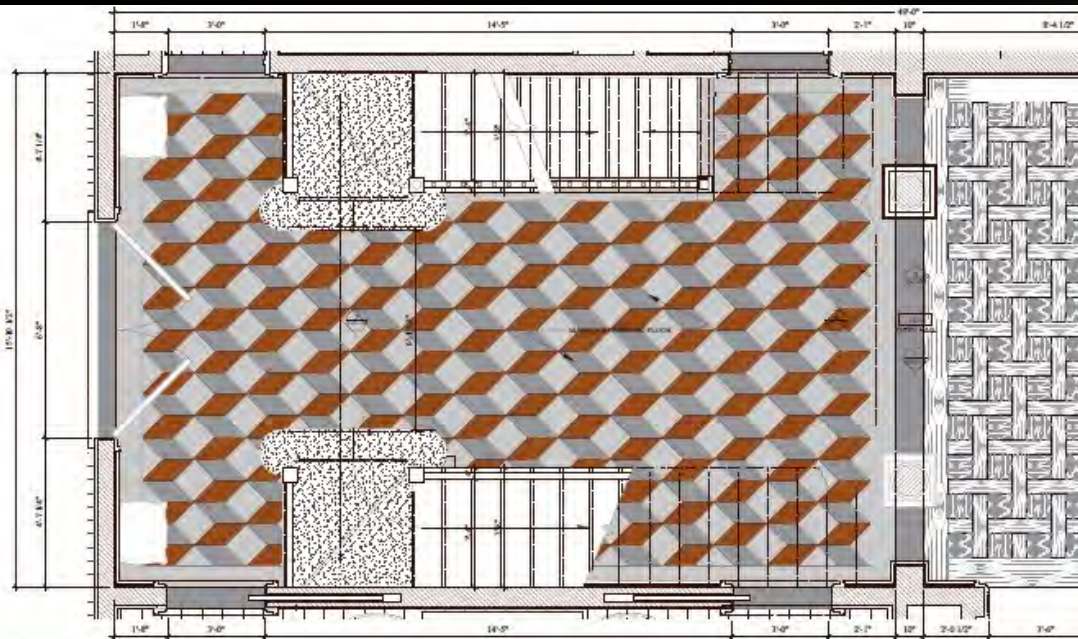
1 PARTIAL FLOOR PLAN @ ENTRY HALL 1/2" = 1'-0"
