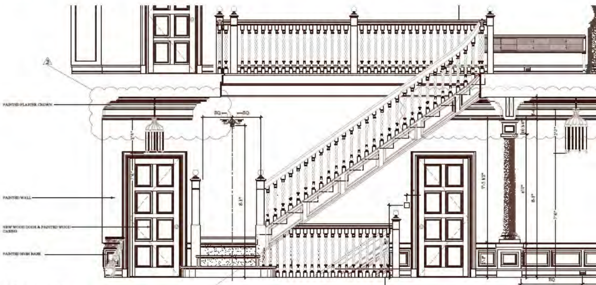
2 SOUTH ELEVATION @ ENTRY HALL 1/2" = 1'-0"
