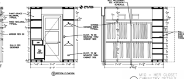
B CLOSET ELEVATION
