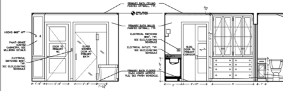
12 PRIMARY BATH WEST INTERIOR ELEVATION SCALE: 1/2"=1'-0"
