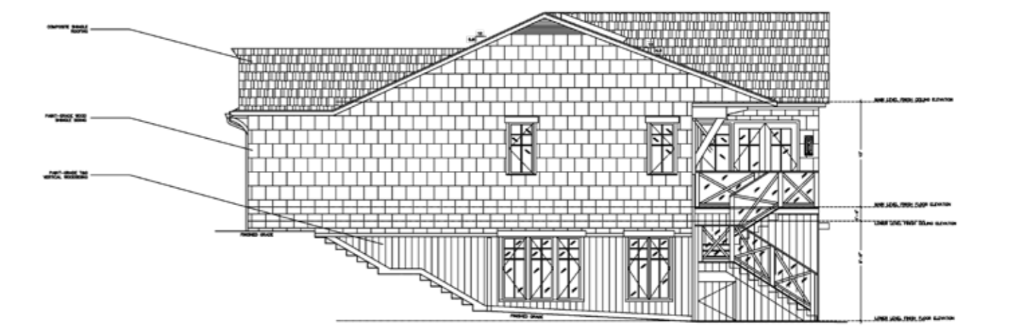
1 EAST EXTERIOR ELEVATION SCALE: 1/8"=1'-0"
