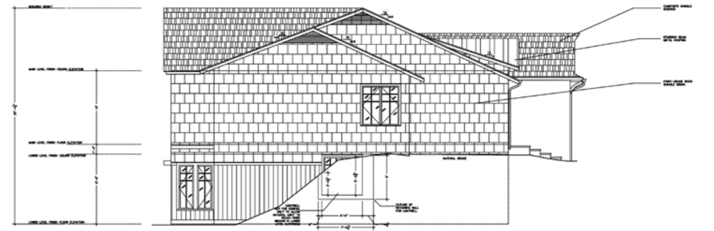
2 REAR EXTERIOR ELEVATION SCALE: 1/8"=1'-0"
