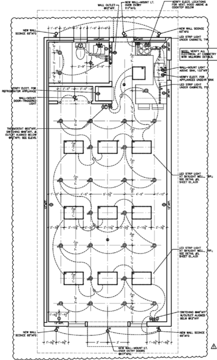
2 LIGHTING AND ELECTRICAL PLAN SCALE: 3/8"=1'-0"
