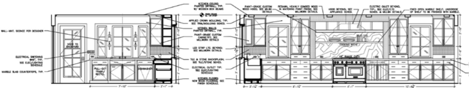
4 KITCHEN EAST INTERIOR ELEVATION SCALE: 1/2"=1'-0"
