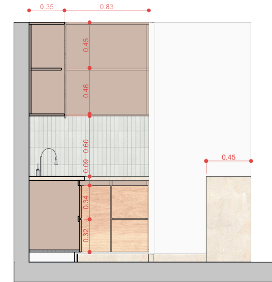
Transverse Section of the Kitchen
