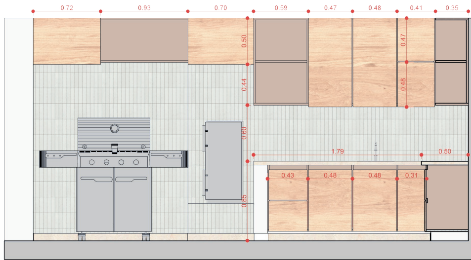
Longitudinal Section of the Kitchen
