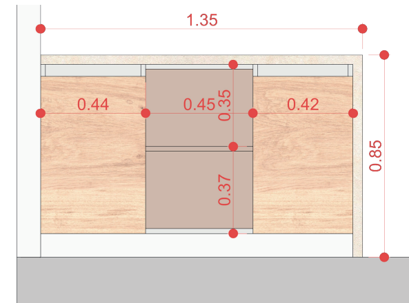
Front View of the Kitchen Counter
