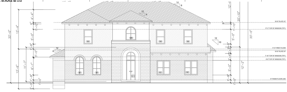
1 FRONT ELEVATION
