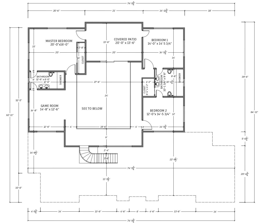
FIRST FLOOR
