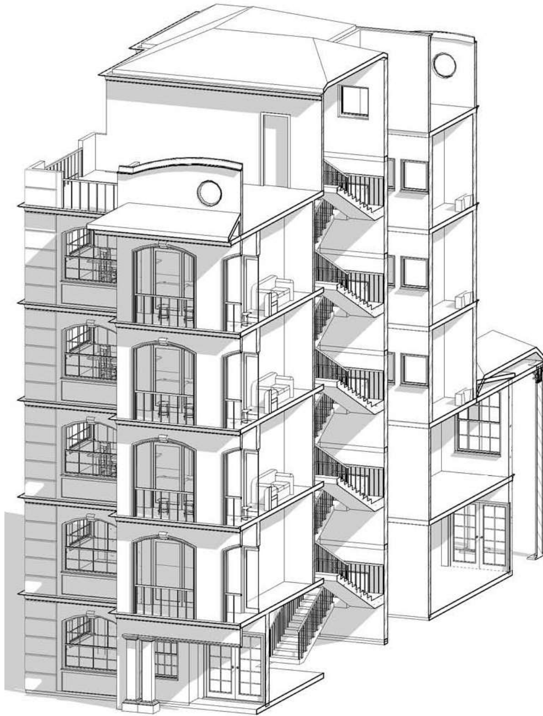
Isometric Section
