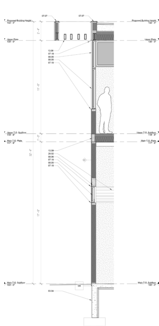
Detail Wall Section
