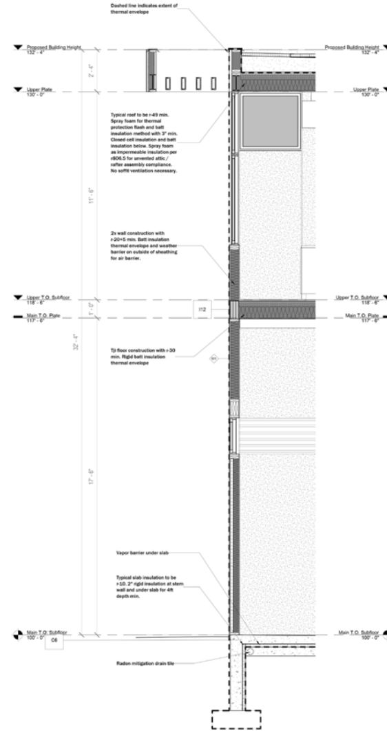
IECC Wall Section
