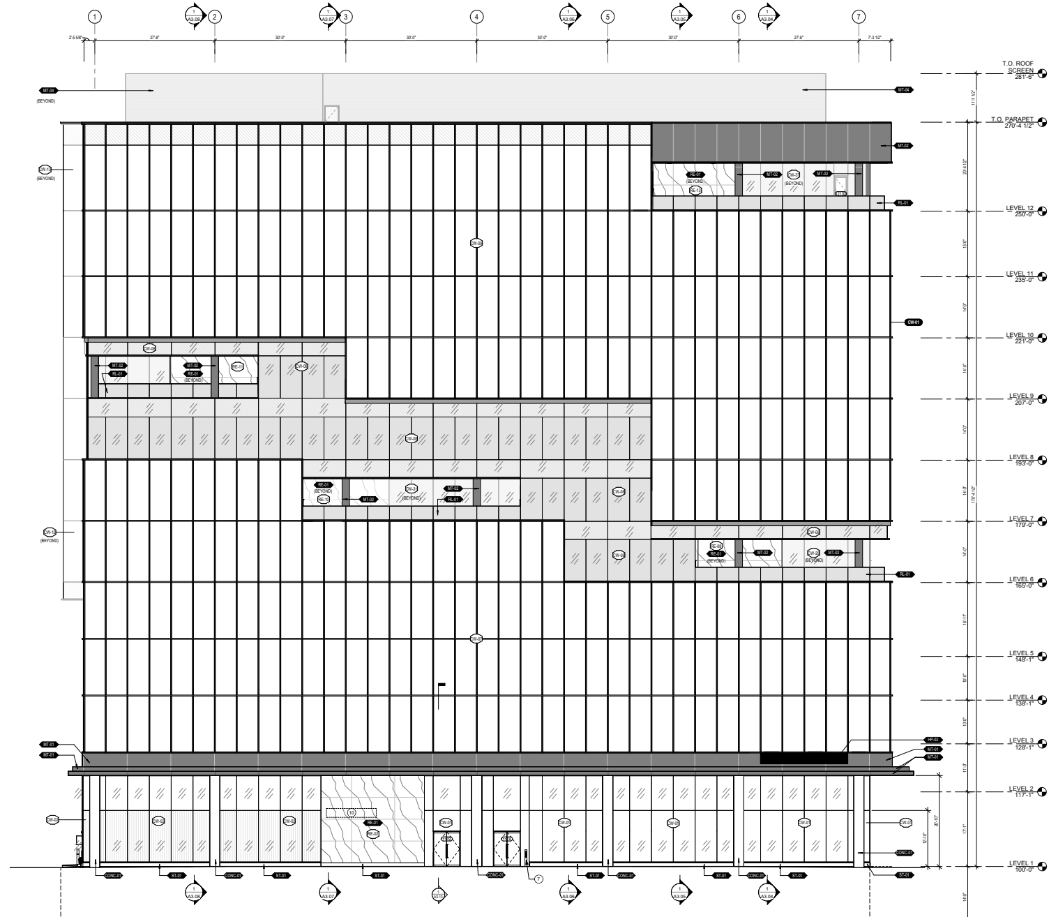
30 West Building Elevation | Construction Documentation - Revit
