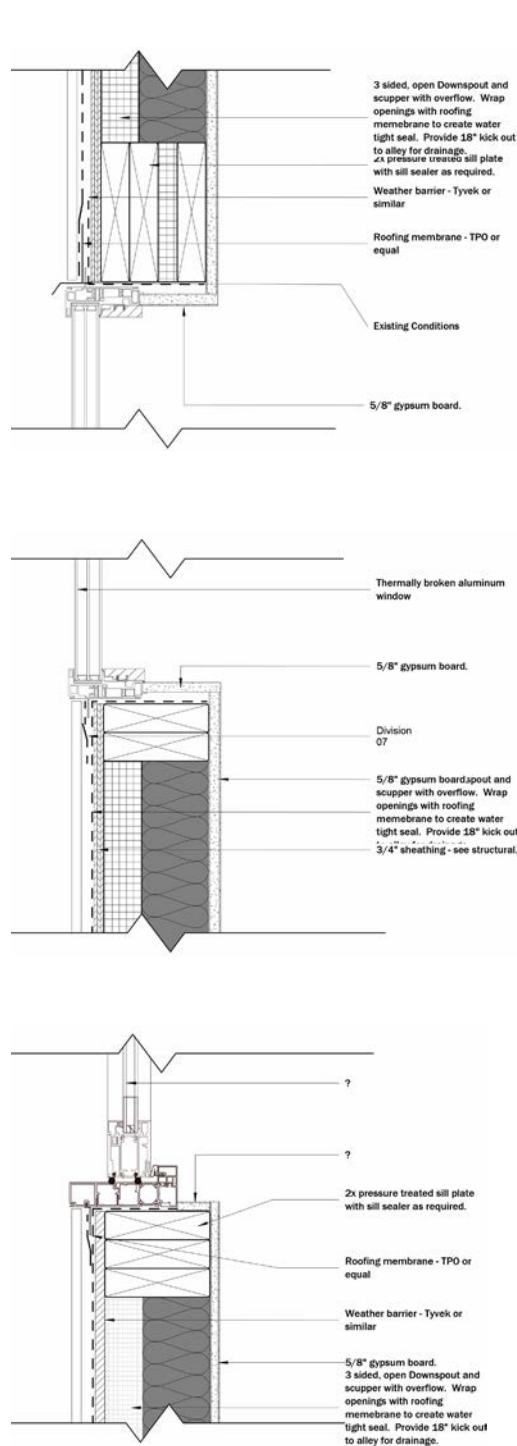
Wall & IECC Sections
