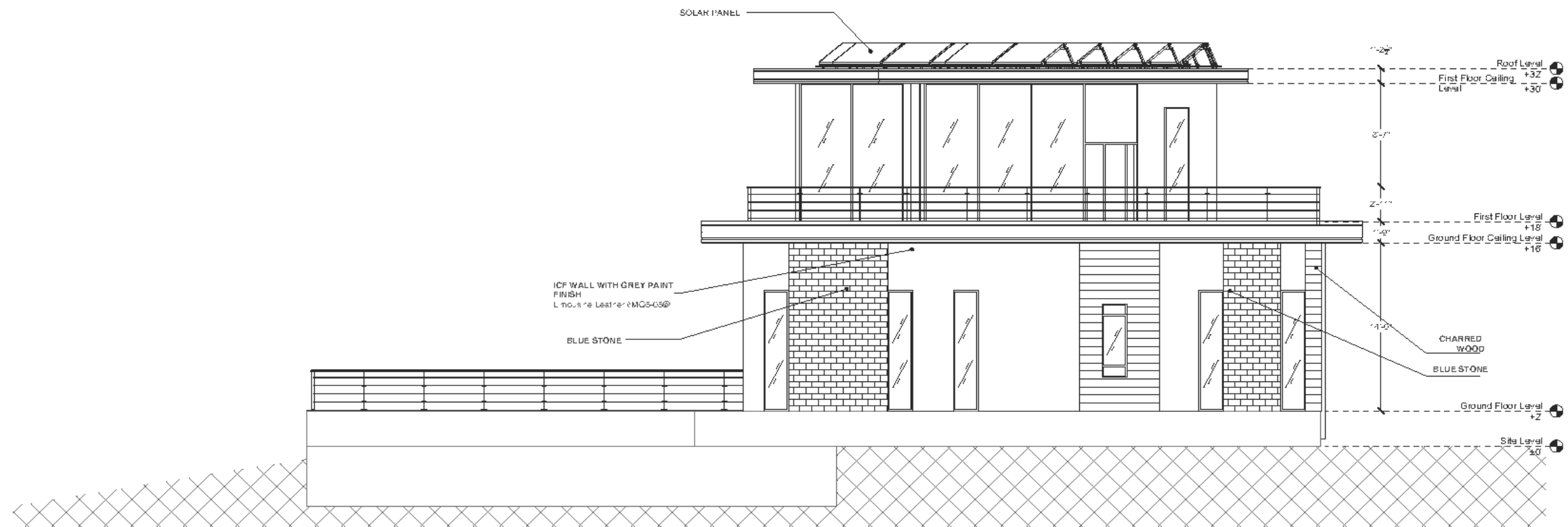
Elevation C
