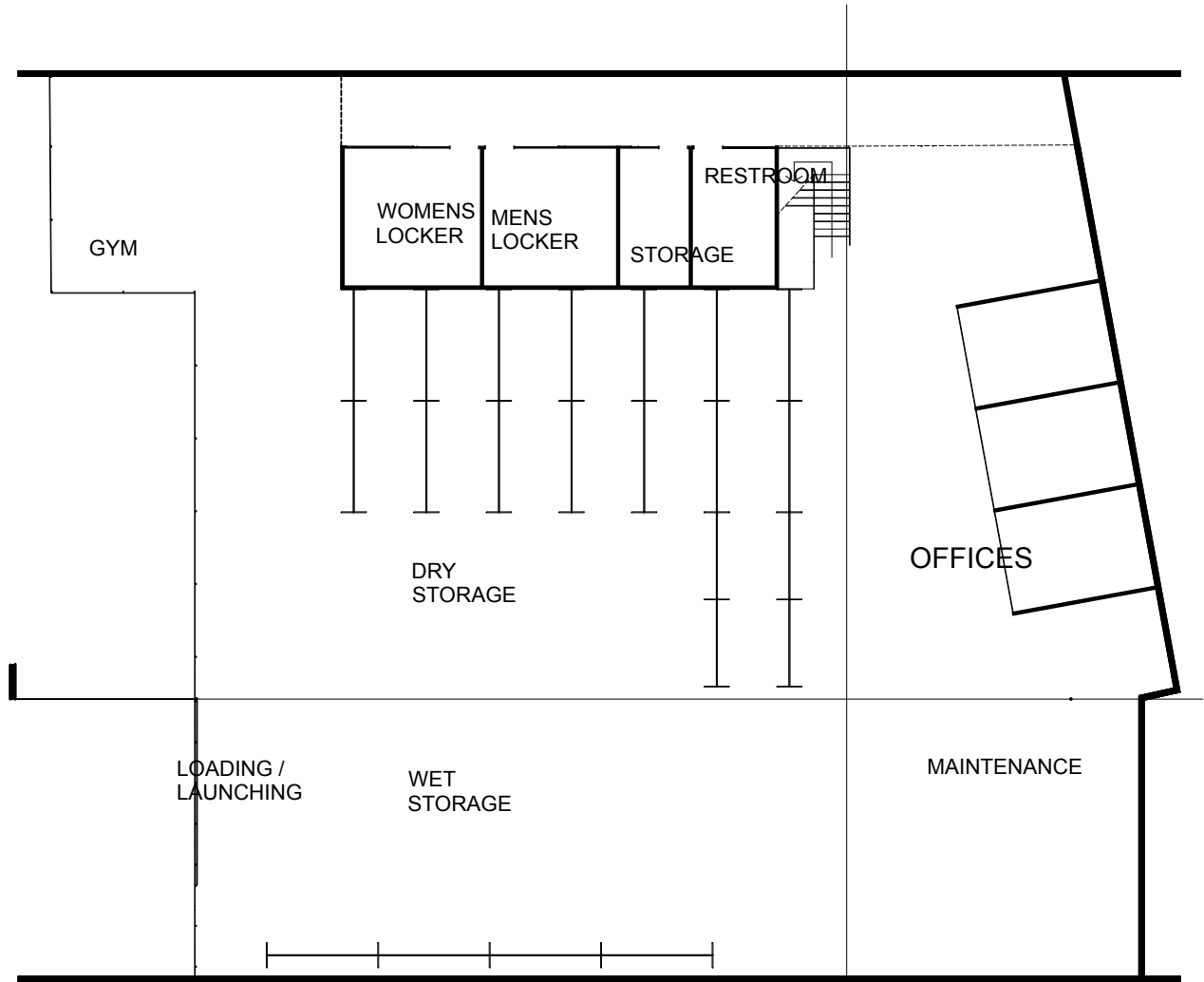
FIRST FLOOR / CIELING PLAN
