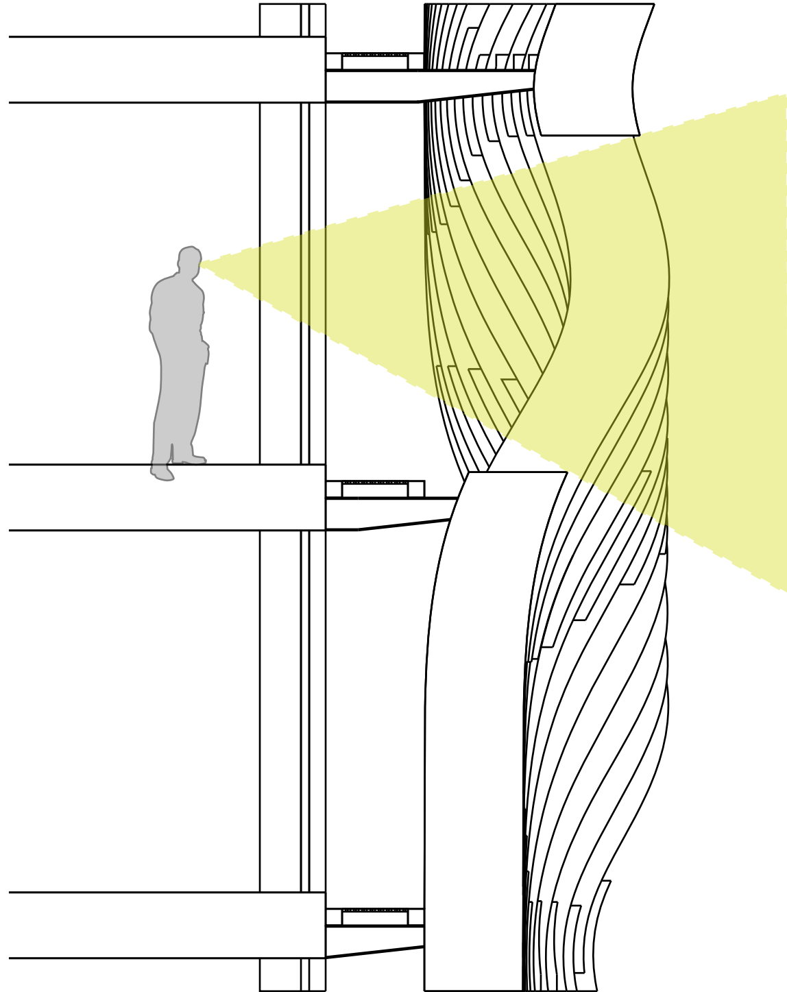
south section
